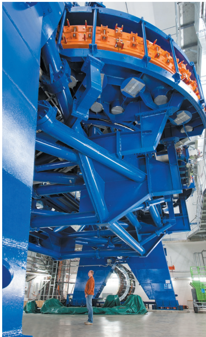
Gantries to direct charged-particle beams weigh as much as 600 tonnes.
