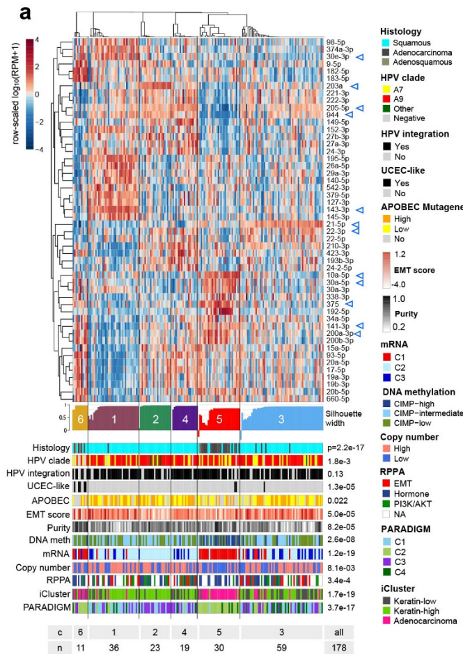
Extended Data Figure 6 | miRNA clusters and miRNA-gene/protein anti-correlations in cervical cancer. a , Unsupervised clustering for miRNA profiles across 178 core-set tumour samples. Top to bottom: a normalized abundance heatmap for the fifty 5p or 3p strands that were highly ranked as differentially abundant by a SAMseq multiclass analysis; a silhouette width profile calculated from the consensus membership matrix; covariates with associated P values; and a summary table of the number of samples in each cluster. The scale bar shows row-scaled \log_{10}(\text{RPM} + 1) normalized abundances. Blue triangles mark selected cancer-associated miRs that were both differentially abundant across the
