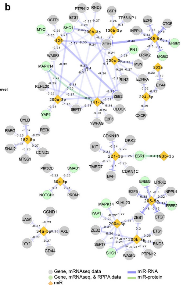
subtypes and abundant in at least one subtype. b , Subnetworks of potential targeting relationships for a subset of miRNAs, as significance-thresholded ( \text{FDR} < 0.05 ) miRNA–mRNA and miRNA–protein anti-correlations that are supported by functionally validated publications. For genes (nodes), colour distinguishes those that are only present in mRNA data (grey) from those that are present in both mRNA and RPPA data (green). Edges represent anti-correlations, and colour distinguishes anti-correlations between miRNA and mRNA (blue); and miRNA and unphosphorylated protein (green). In the n = 178 core-set cohort, no correlations satisfying \text{FDR} < 0.05 were reported between miRNA and phosphorylated protein.
