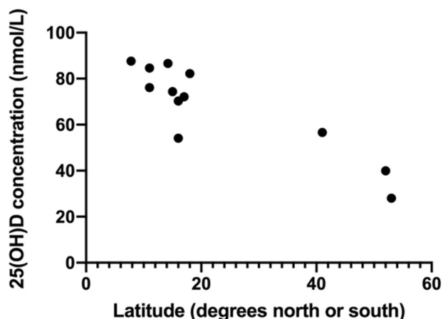
Fig. 2 Relationship between vitamin concentration [25(OH)D] and latitude in the African-Caribbean population. Note: 95% confidence interval: -1.210, -0.577, p < 0.0001 . Mean 25(OH)D concentration of 67.8 nmol/L, 95% CI (57.9, 77.6) from the 12 papers ( n = 2974 , globally) included in the meta-analysis on 25(OH)D concentration [17, 21, 33–39, 42–44]. Latitude reported by author or estimated. Additional unpublished data was provided by some authors.
