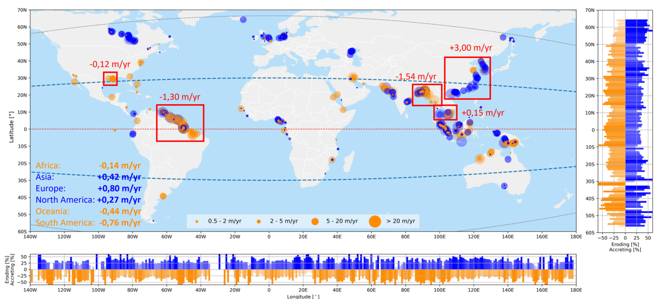
Fig. 2 | Global hot spots of muddy coast erosion and accretion; the orange (blue) circles indicate erosion (accretion) for the four relevant coastline dynamic classifications (see legend). The bar plots to the right and at the bottom
