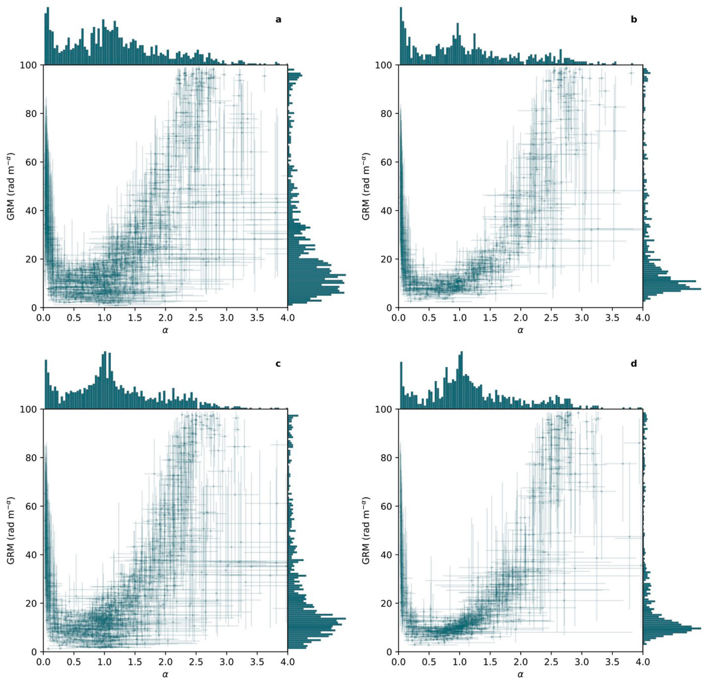
Extended Data Fig. 7 | Generalized rotation measure and wavelength dependencies inferred from four simulations of propagation through two Faraday screens. Distributions of the recovered median a-posteriori (with 68% confidence intervals shown by the errorbars) generalized rotation measure and wavelength dependence inferred from four simulations of incoherent propagation through two Faraday screens. Top row depicts the results from
