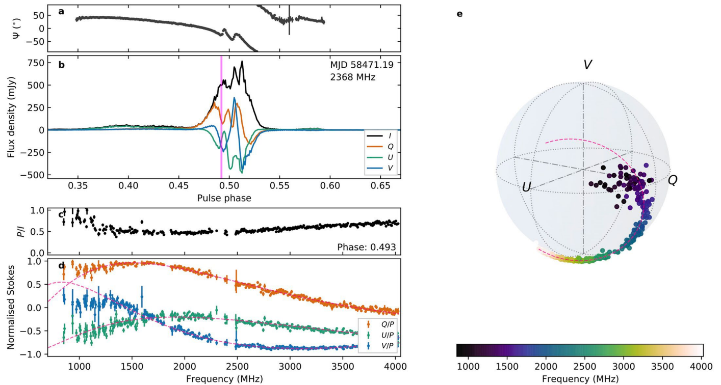
Extended Data Fig. 5 | Example where our Faraday conversion model failed to fit low-frequency variations in XTE J1810-197. Linear polarization PA and 1-\sigma uncertainties (a) along with the time- and frequency-averaged polarization profile (b) of XTE J1810-197 detected on 19 December 2018, where the black, orange, green and blue lines respectively correspond to the total intensity ( I ), two linear polarizations ( Q and U ) and the circular polarization ( V ). The vertical
