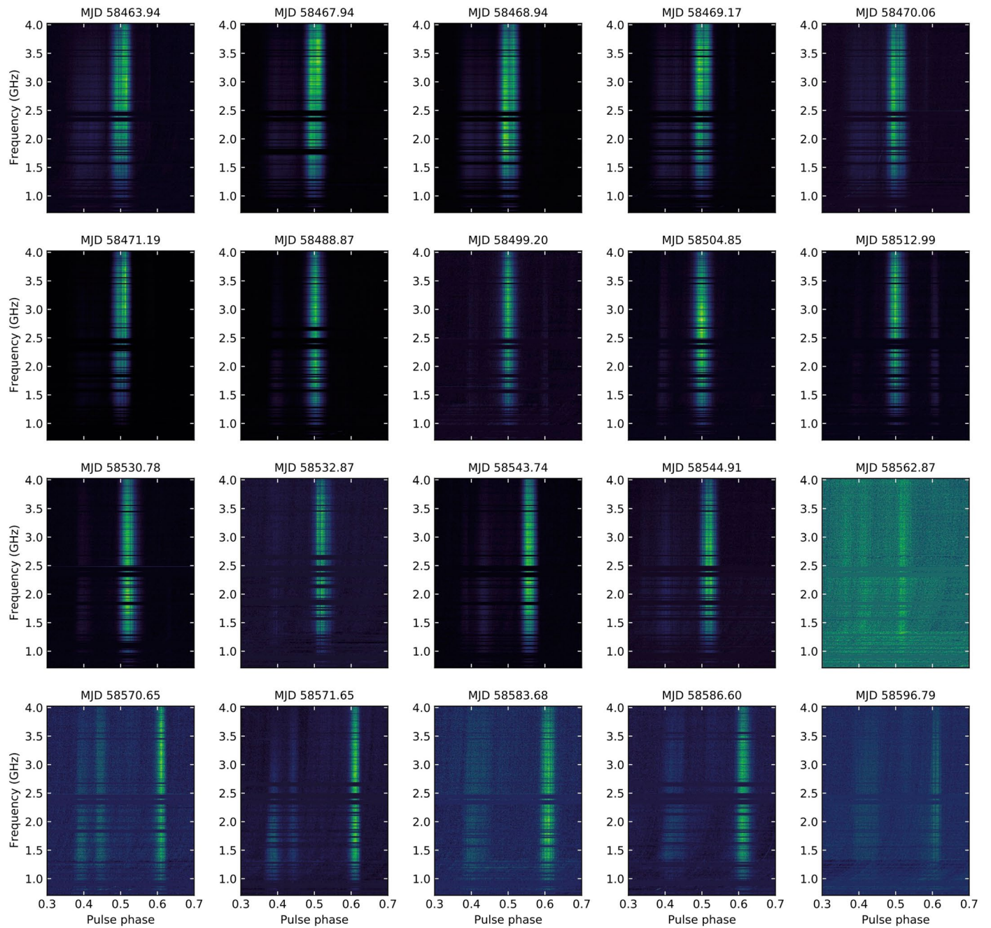
Extended Data Fig. 2 | Total intensity spectrum of XTE J1810-197 over time. Normalized total intensity of XTE J1810-197 as a function of pulse phase and observing frequency. Horizontal bands in each panel correspond to channels that were excised due to contamination by radio frequency interference.
