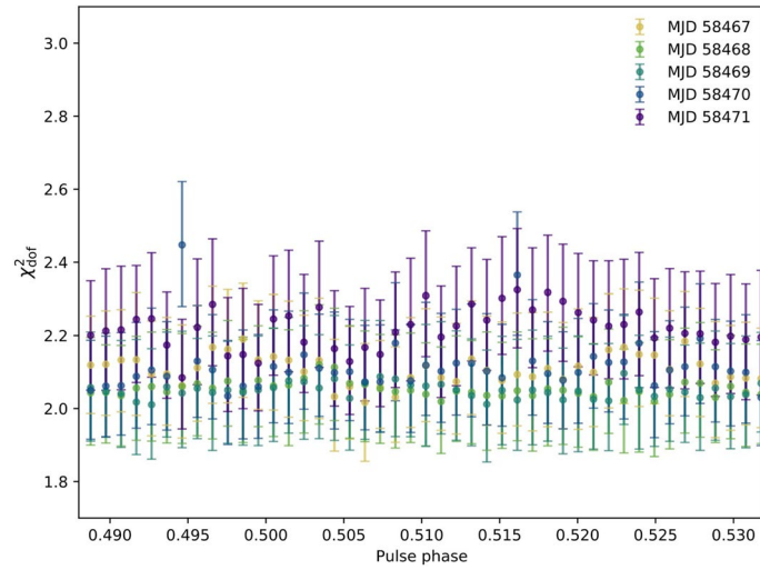
Extended Data Fig. 4 | Reduced chi-square distributions from Faraday conversion fits to XTE J1810–197. Recovered median (points) and 68 percent intervals (error bars) of the reduced chi-square statistic ( \chi^2_{\text{dof}} ) after subtracting
