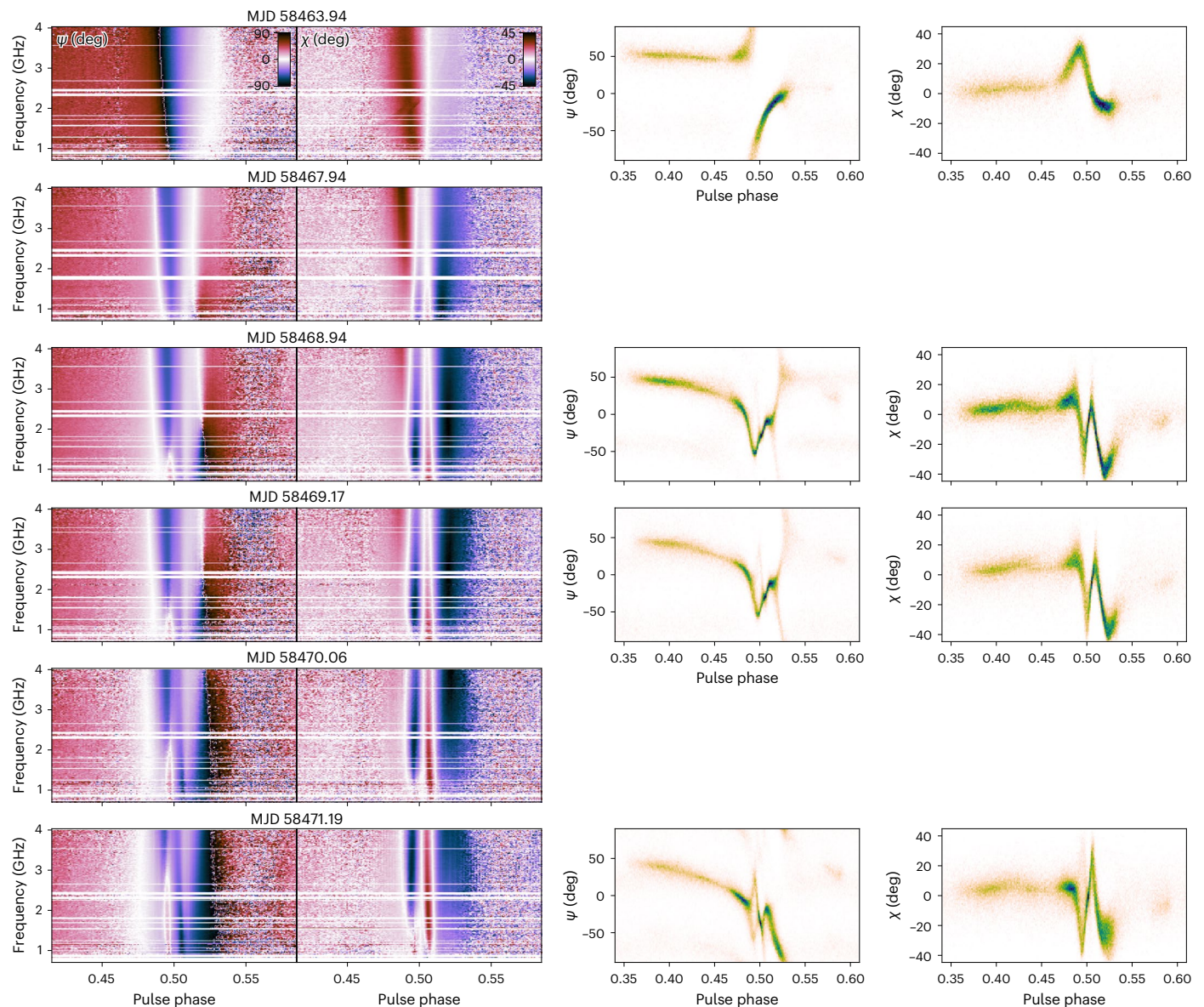
Fig. 2 | Evolution of the phase- and frequency-resolved polarization properties of XTE J1810–197. Left-hand panels show the linear polarization PA ( \psi , left) and ellipticity angle ( \chi , middle-left) for the Parkes-UWL observations as a function of pulse phase and observing frequency. Blank horizontal lines correspond to frequency channels that were excised due to contamination by RFI.
