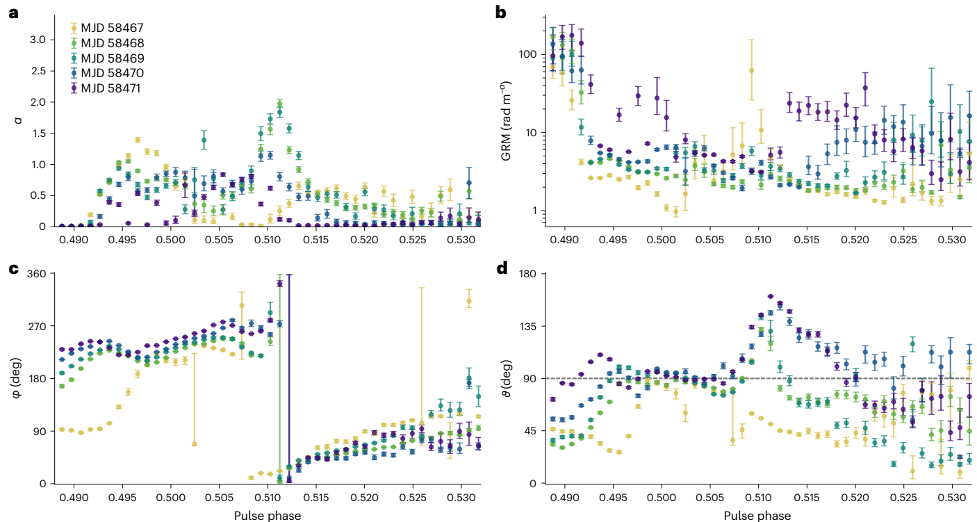
Fig. 4 | Recovered phase-resolved geometric parameters from the polarization conversion model for five Parkes-UWL epochs. a–d, Median a posteriori values (points) 68% confidence intervals (error bars) for the spectral exponent (a), GRM in units of \text{rad m}^{-2} (b), and the longitude (c) and latitude (d) of
