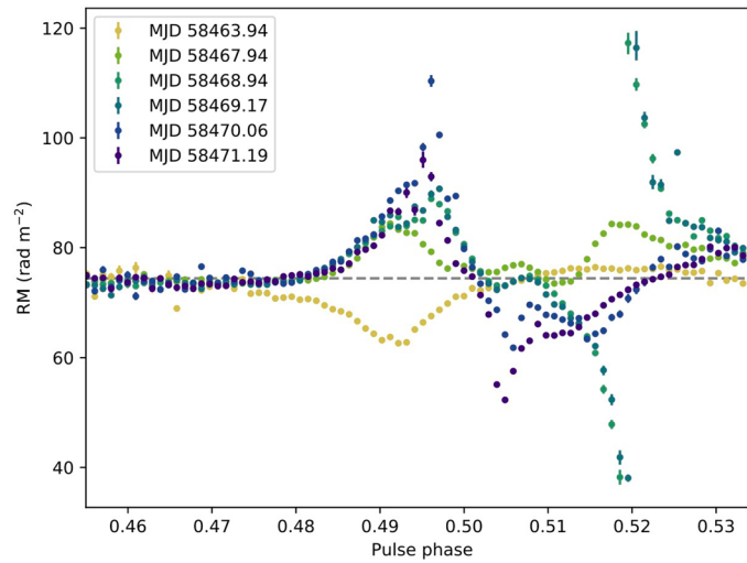
Extended Data Fig. 8 | Phase-resolved rotation measure of XTE J1810–197 in the presence of strong Faraday conversion. Recovered median a-posteriori (points) and 68% confidence intervals (error bars) on the rotation measure of XTE J1810–197 as a function of pulse phase on different epochs. The nominal rotation measure of 74.4 \text{ rad m}^{-2} is indicated by the dashed, horizontal line. Strong
