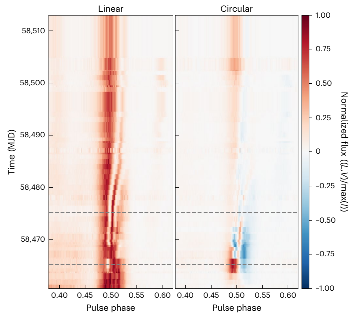
Fig. 1 | Polarization evolution of XTE J1810–197 with time. Linear and circular polarized emission detected by Lovell and Parkes observed at each epoch after averaging in frequency over 1,340–1,724 MHz and 0.07–2.0 h. These data are presented as functions of pulse phase and time. Red and blue colours correspond to positive and negative values, respectively. The initial smooth linear variations across pulse phase and slowly increasing level of positive (left-handed) circular polarization undergo a dramatic change after 13 December 2018 (MJD 58465, lower horizontal line). Sudden reversals in circular handedness correspond to dips in linear intensity due to strong conversion effects. The circular intensity diminishes within roughly 12 days of the 13 December 2018 event (MJD 58477, upper horizontal line). It was then followed by an apparent drift of the linear-to-circular conversion feature to increasingly later phases with time.
