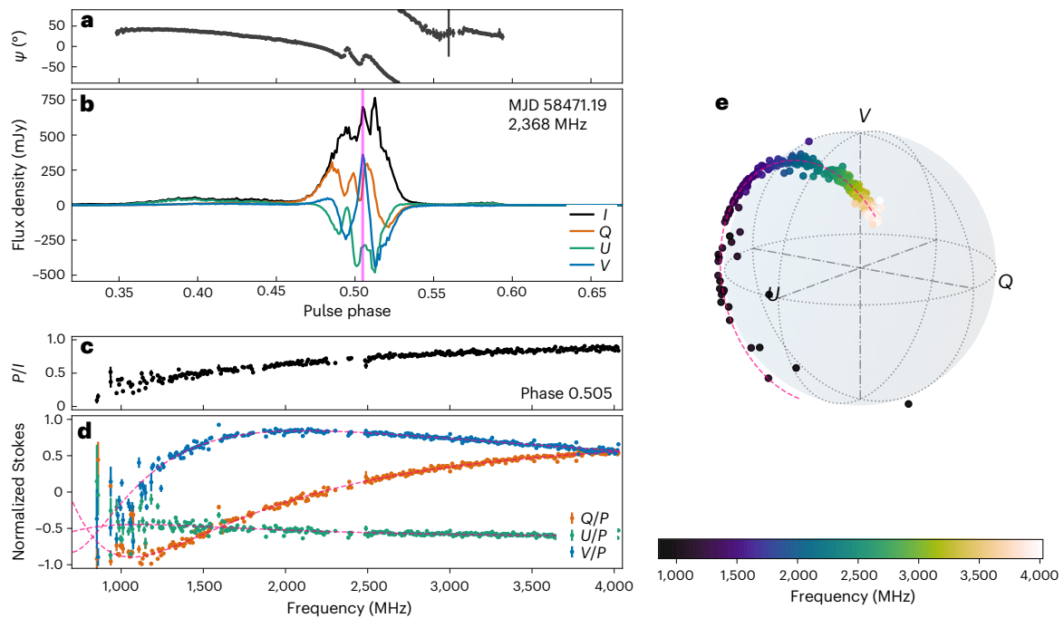
Fig. 3 | Example detection of linear-to-circular conversion in XTE J1810–197. a, b , Linear polarization PA and 1-\sigma uncertainties ( a ) along with the time- and frequency-averaged polarization profile ( b ) of XTE J1810–197 detected on 19 December 2018, where the black, orange, green and blue lines, respectively, correspond to the total intensity ( I ), two linear polarizations ( Q and U ) and the circular polarization ( V ). c, d , The vertical magenta line indicates the phase bin (0.505 in this plot) for which we plot the corresponding time-averaged
