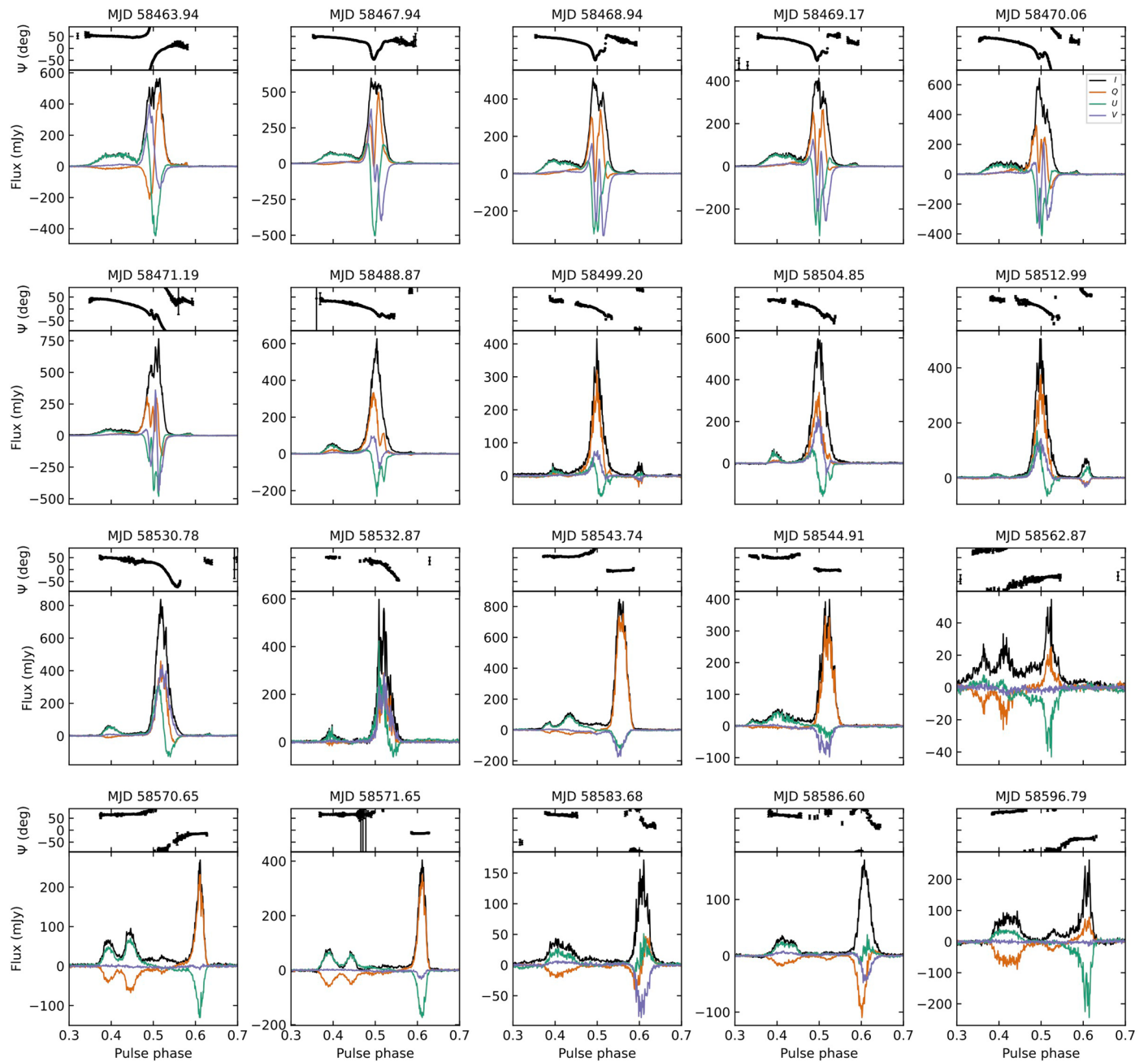
Extended Data Fig. 1 | Evolving polarization profile of XTE J1810-197. Time- and frequency-averaged polarization profile and linear polarization position angle of XTE J1810-197 observed by Parkes from MJD 58463 to 58596. Black, orange, green and purple lines correspond to Stokes I , Q , U and V respectively.
