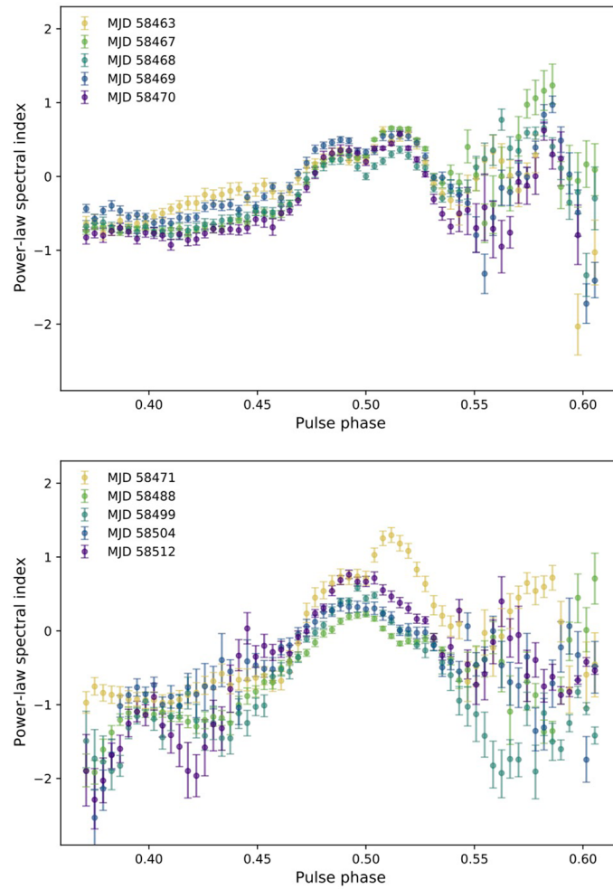
Extended Data Fig. 3 | Phase-resolved spectral index evolution of XTE J1810–197. Median a-posteriori values (points) 68% confidence intervals (error bars) for the spectral indices measured from power-law fits to the total intensity profile. Results from subsequent epochs are represented by the different colors.
